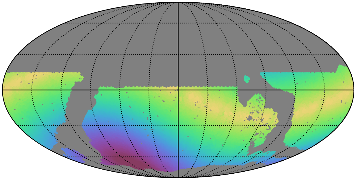
roll_pause_mjdp270_v3.4_10yrs WFD u band: Max solarElong
