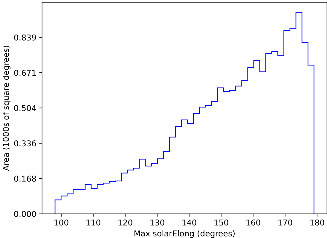
roll_pause_mjdp270_v3.4_10yrs WFD u band: Max solarElong
