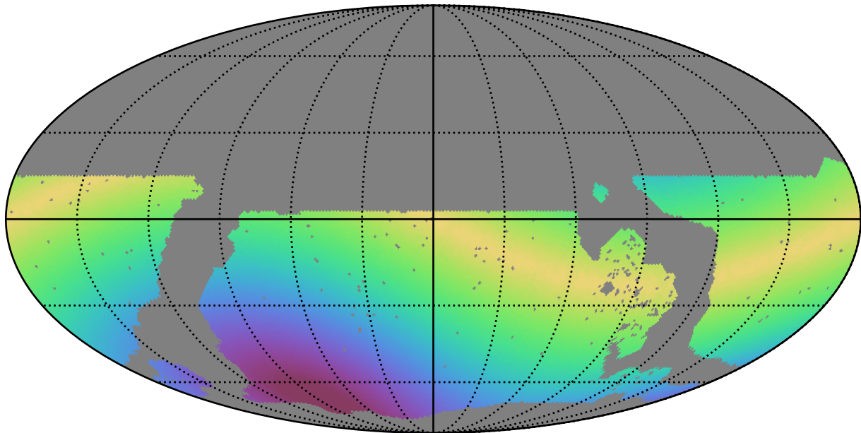
roll_pause_mjdp270_v3.4_10yrs WFD r band: Max solarElong
