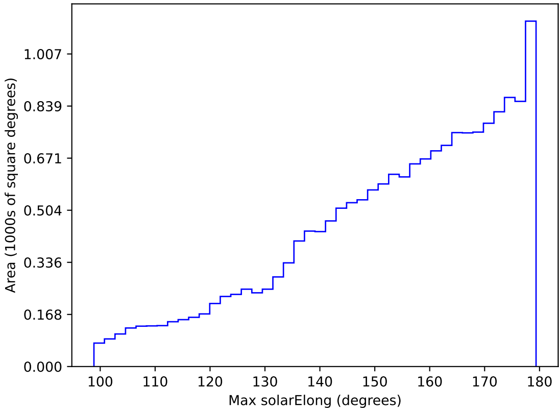
roll_pause_mjdp270_v3.4_10yrs WFD r band: Max solarElong
