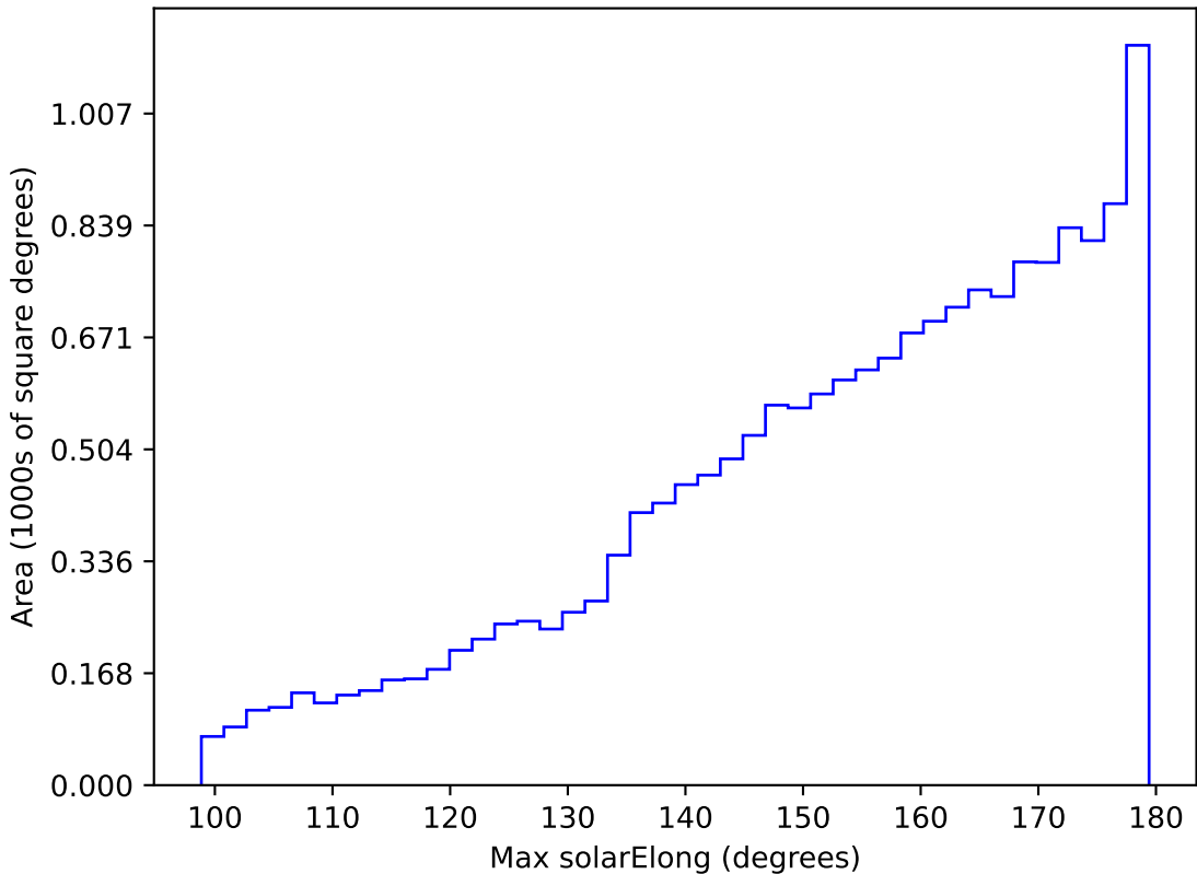
roll_pause_mjdp270_v3.4_10yrs WFD i band: Max solarElong
