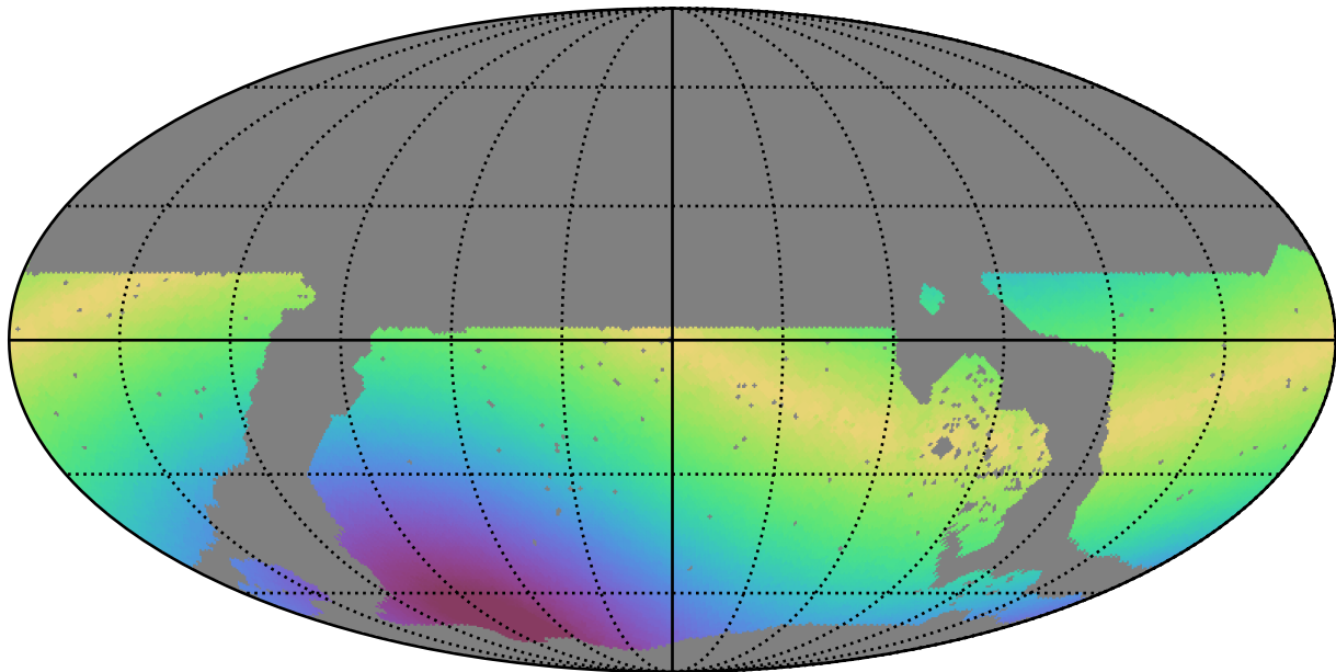
roll_pause_mjdp270_v3.4_10yrs WFD g band: Max solarElong
