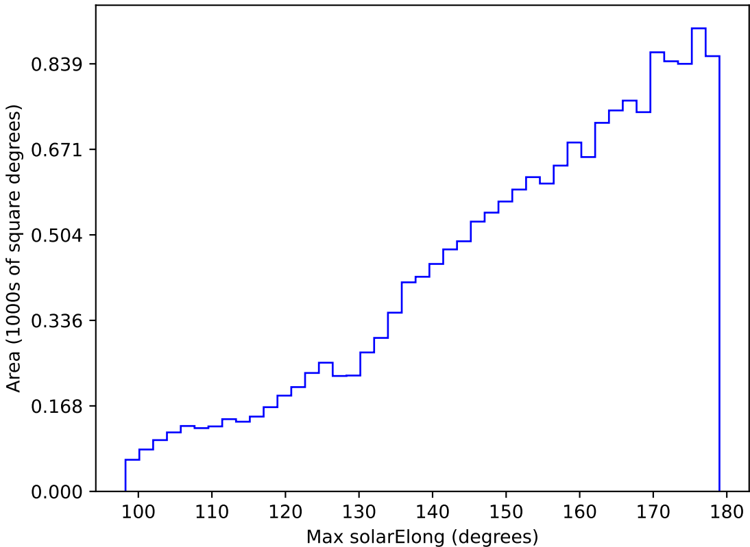
roll_pause_mjdp270_v3.4_10yrs WFD g band: Max solarElong
