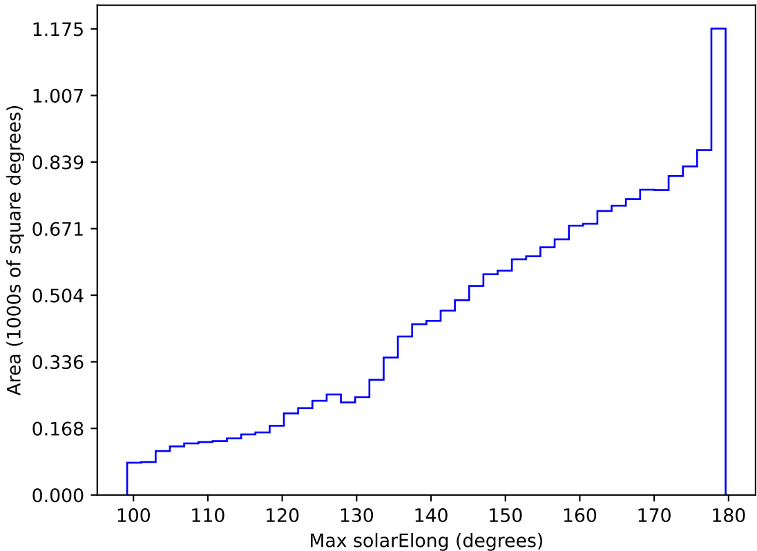
roll_pause_mjdp270_v3.4_10yrs WFD all bands: Max solarElong
