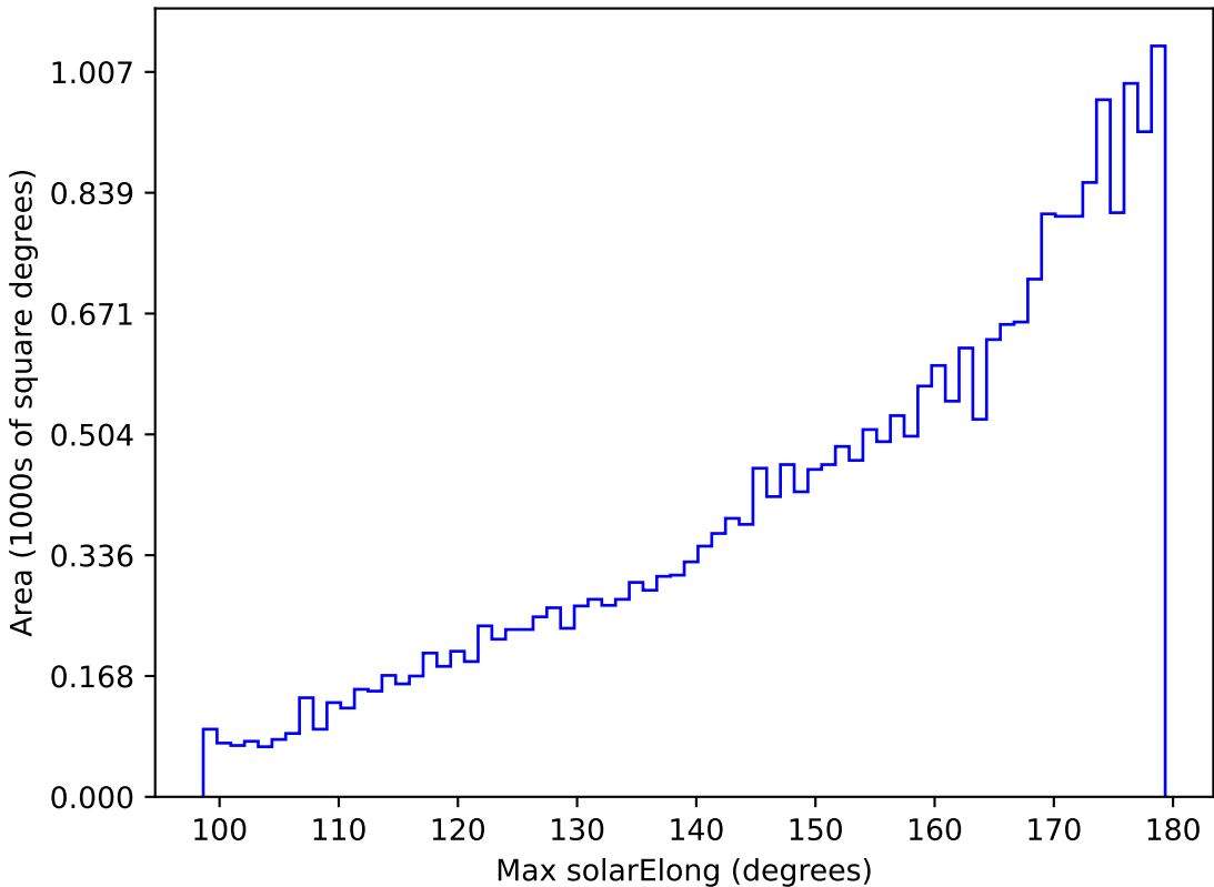
roll_pause_mjdp270_v3.4_10yrs All sky z band: Max solarElong
