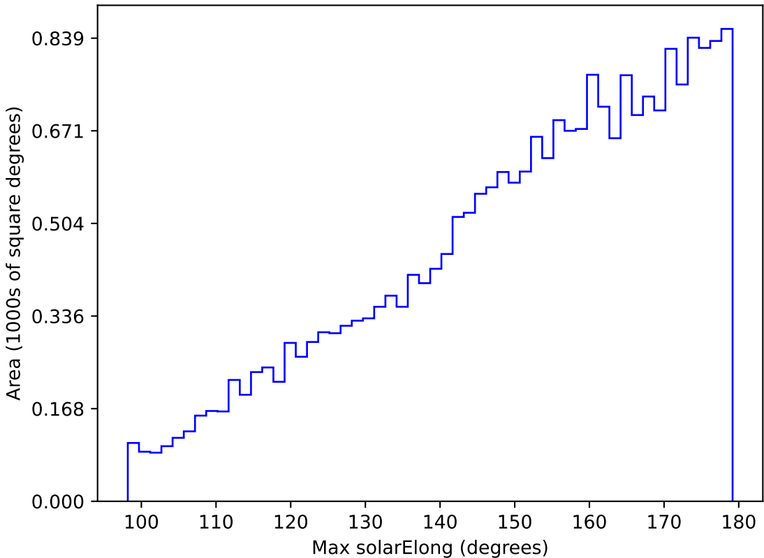
roll_pause_mjdp270_v3.4_10yrs All sky y band: Max solarElong
