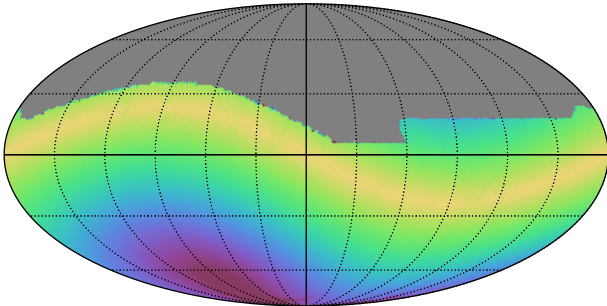
roll_pause_mjdp270_v3.4_10yrs All sky r band: Max solarElong
