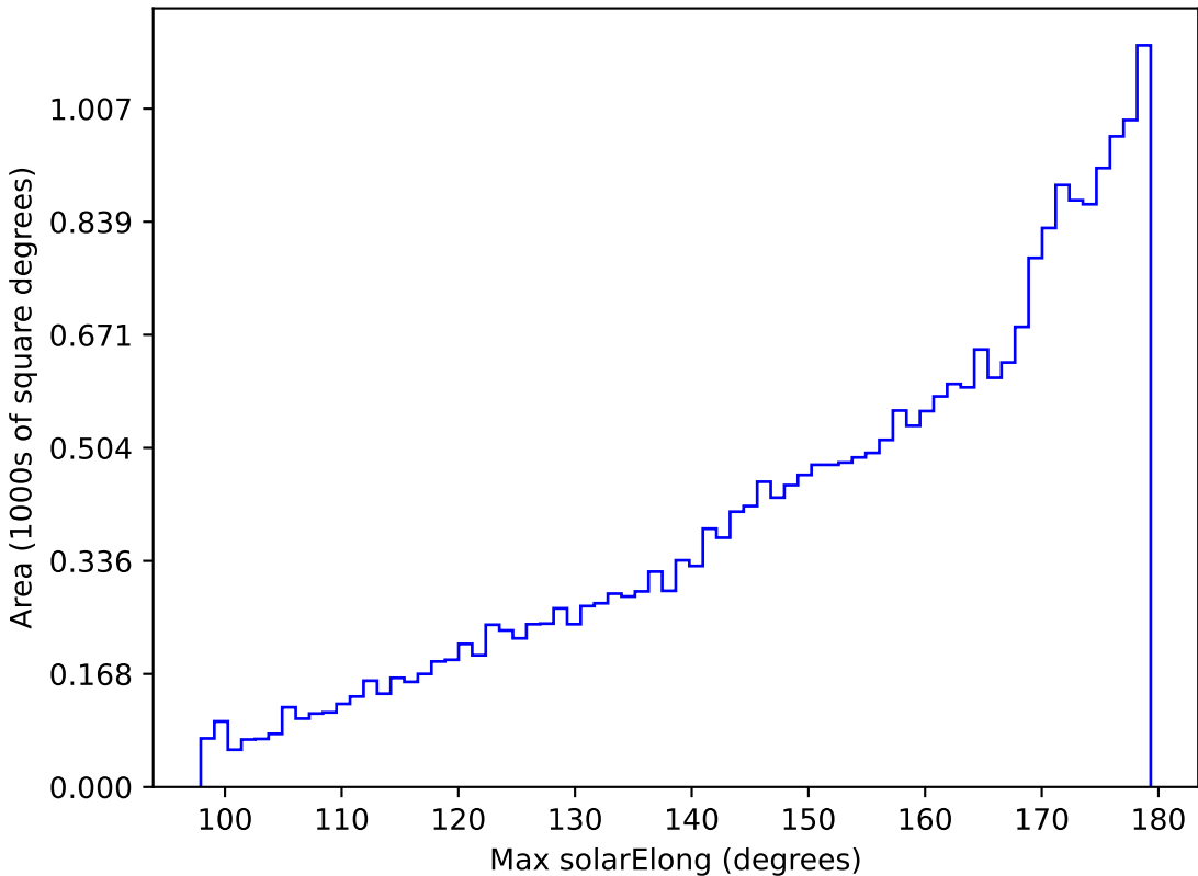
roll_pause_mjdp270_v3.4_10yrs All sky r band: Max solarElong
