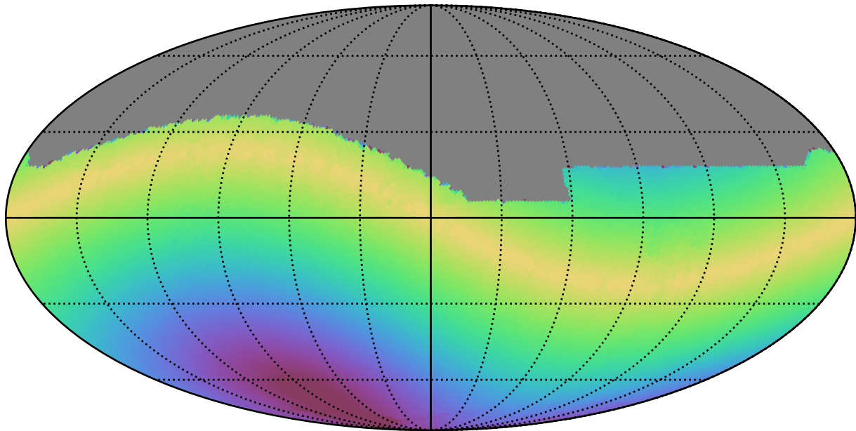
roll_pause_mjdp270_v3.4_10yrs All sky i band: Max solarElong
