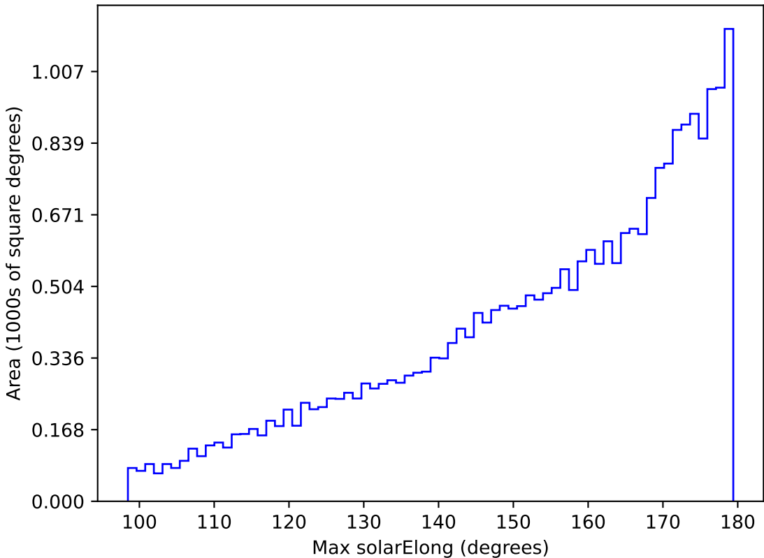
roll_pause_mjdp270_v3.4_10yrs All sky i band: Max solarElong
