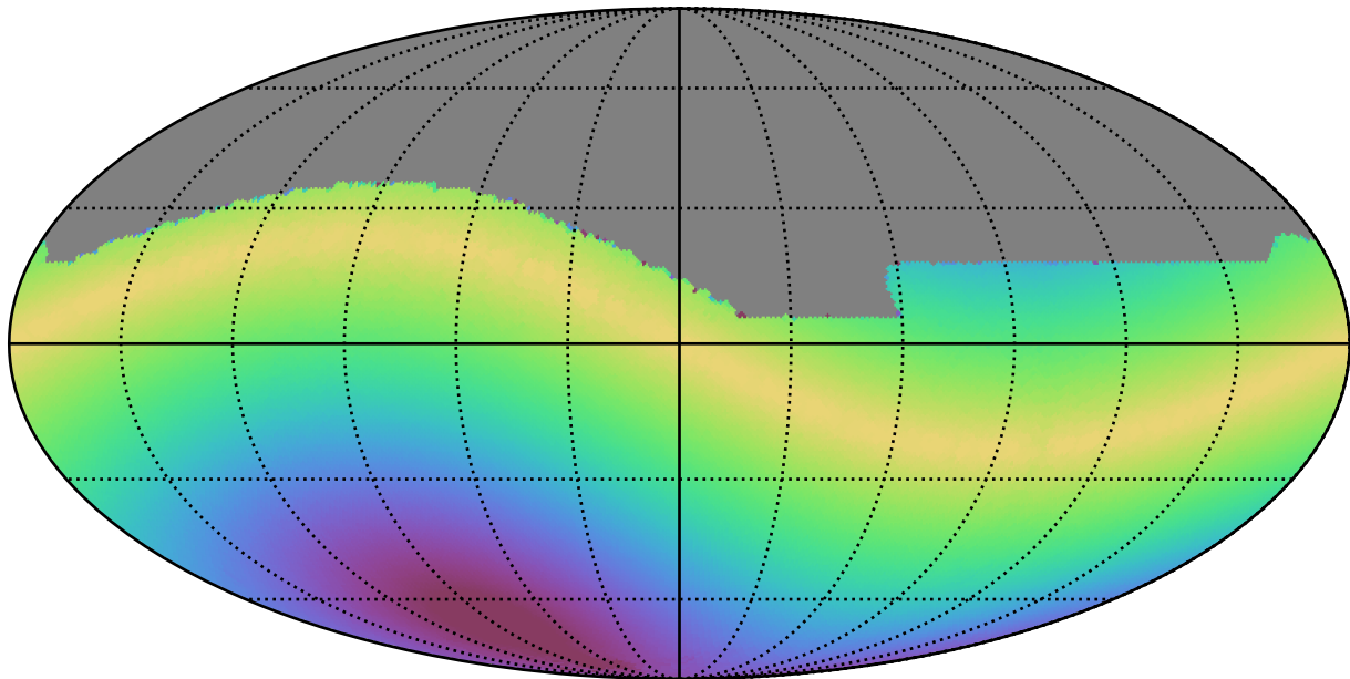
roll_pause_mjdp270_v3.4_10yrs All sky all bands: Max solarElong
