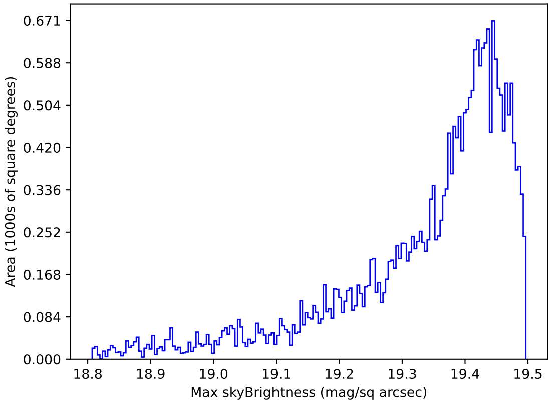
roll_pause_mjdp270_v3.4_10yrs Yr 1 z band: Max skyBrightness
