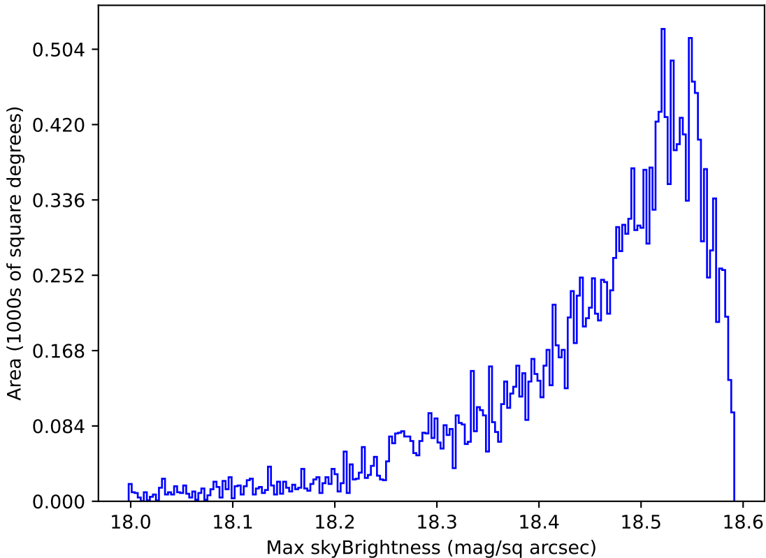
roll_pause_mjdp270_v3.4_10yrs Yr 1 y band: Max skyBrightness
