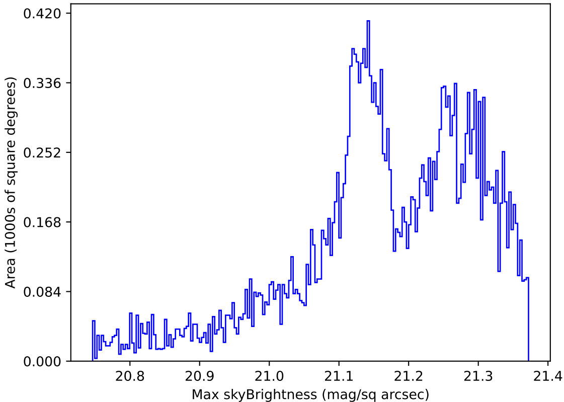
roll_pause_mjdp270_v3.4_10yrs Yr 1 r band: Max skyBrightness
