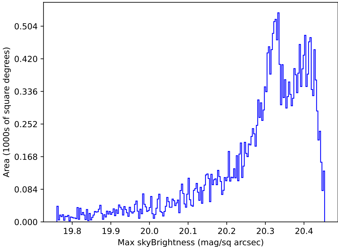
roll_pause_mjdp270_v3.4_10yrs Yr 1 i band: Max skyBrightness
