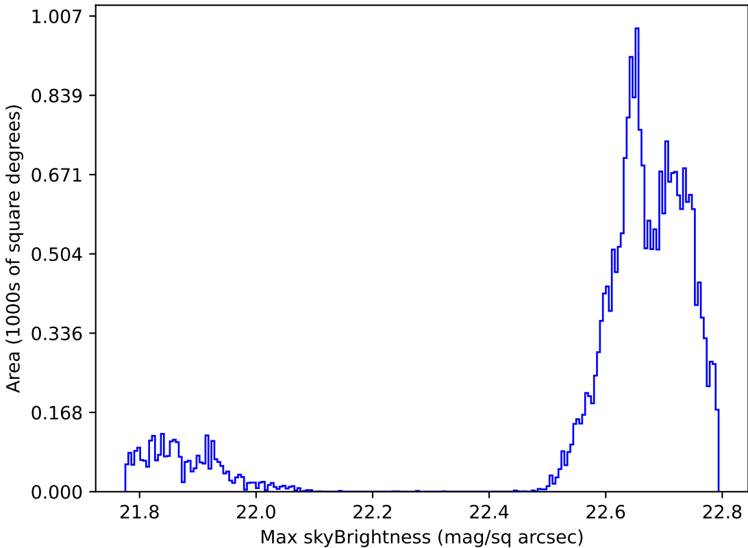
roll_pause_mjdp270_v3.4_10yrs Yr 1 all bands: Max skyBrightness
