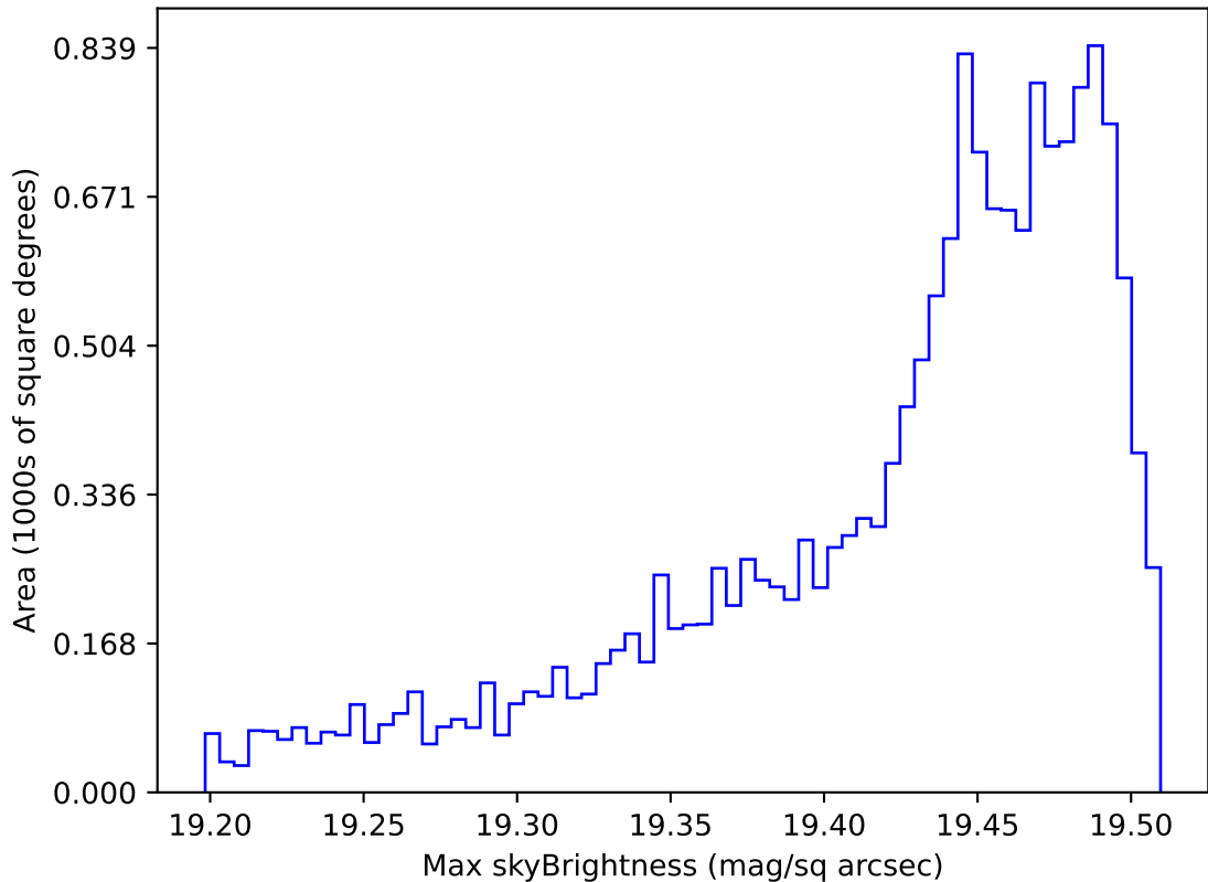
roll_pause_mjdp270_v3.4_10yrs WFD z band: Max skyBrightness
