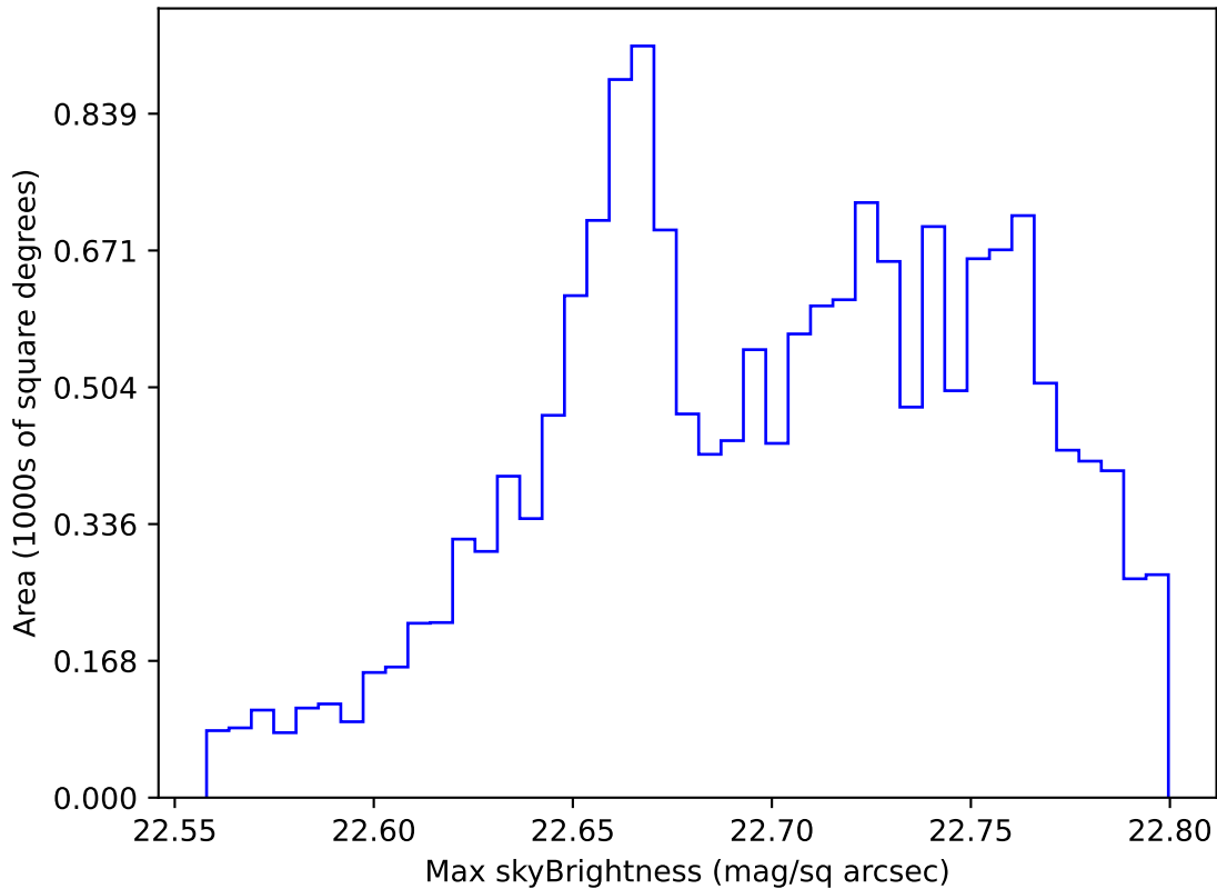
roll_pause_mjdp270_v3.4_10yrs WFD u band: Max skyBrightness
