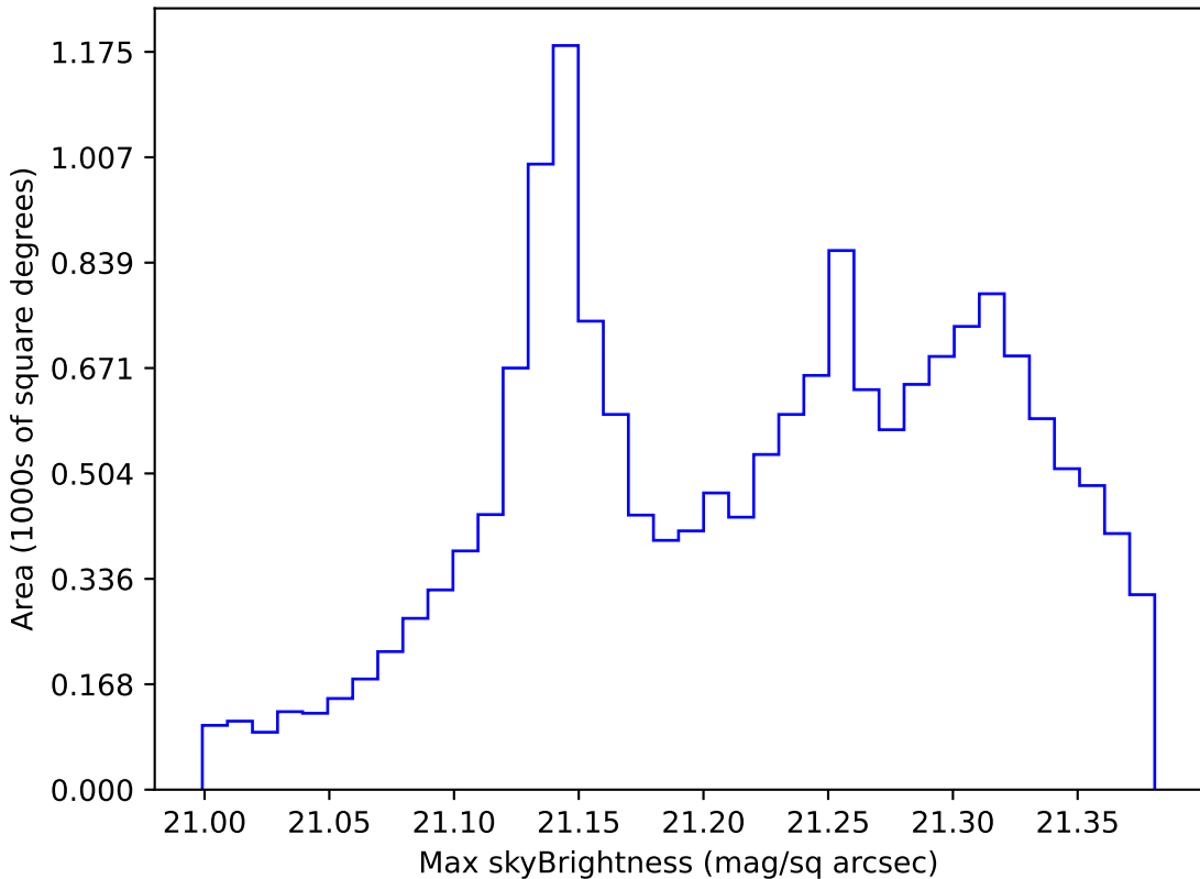
roll_pause_mjdp270_v3.4_10yrs WFD r band: Max skyBrightness
