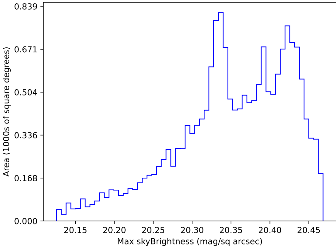
roll_pause_mjdp270_v3.4_10yrs WFD i band: Max skyBrightness
