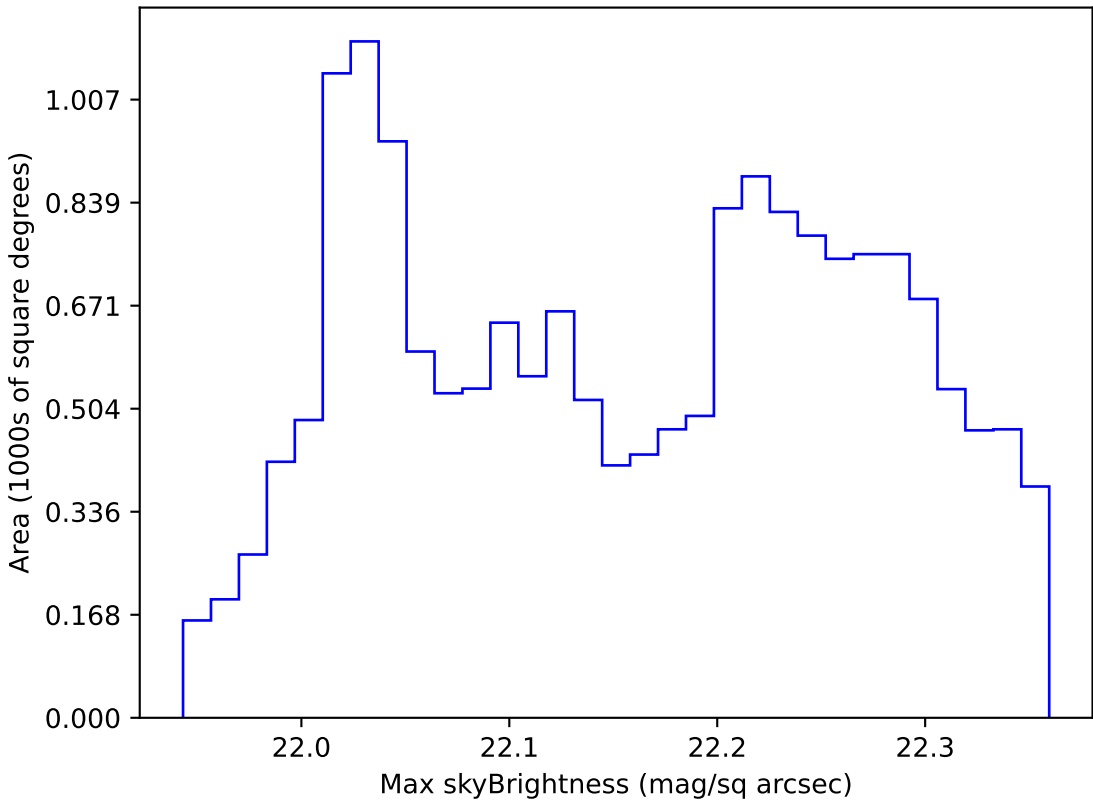
roll_pause_mjdp270_v3.4_10yrs WFD g band: Max skyBrightness
