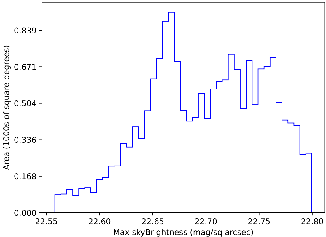
roll_pause_mjdp270_v3.4_10yrs WFD all bands: Max skyBrightness
