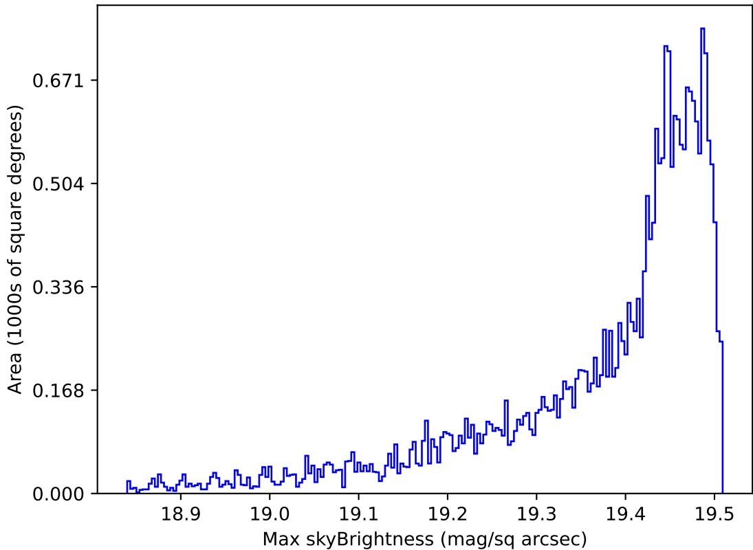
roll_pause_mjdp270_v3.4_10yrs All sky z band: Max skyBrightness
