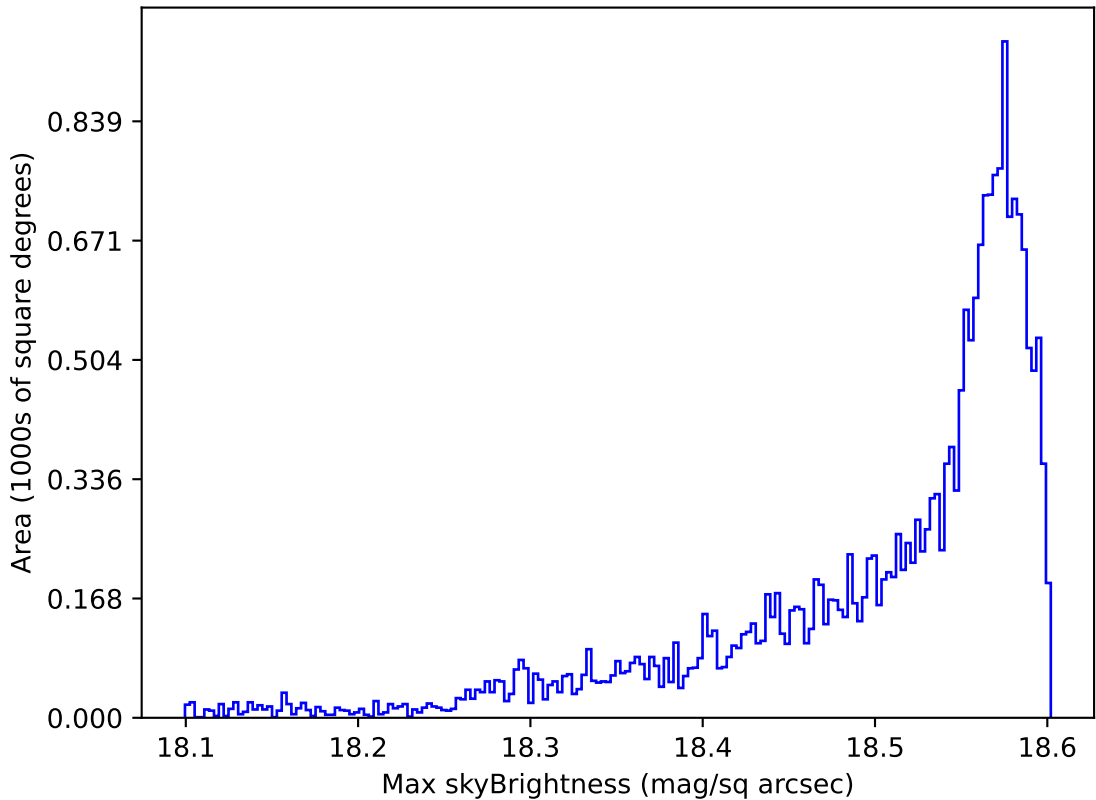
roll_pause_mjdp270_v3.4_10yrs All sky y band: Max skyBrightness
