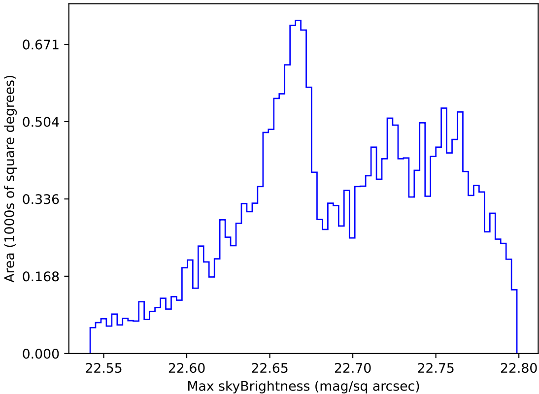
roll_pause_mjdp270_v3.4_10yrs All sky u band: Max skyBrightness
