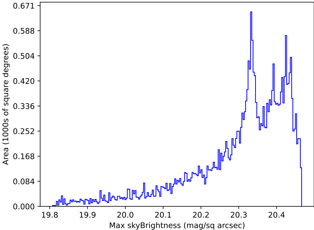
roll_pause_mjdp270_v3.4_10yrs All sky i band: Max skyBrightness
