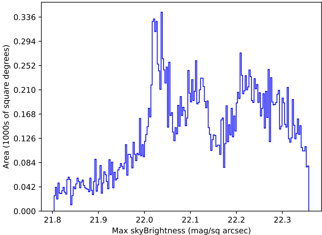
roll_pause_mjdp270_v3.4_10yrs All sky g band: Max skyBrightness
