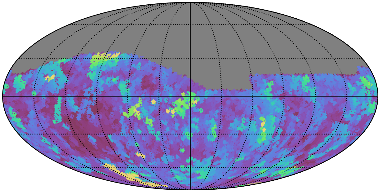
roll_pause_mjdp270_v3.4_10yrs Yr 1 z band: Max seeingGeom
