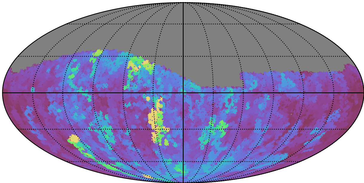
roll_pause_mjdp270_v3.4_10yrs Yr 1 g band: Max seeingEff
