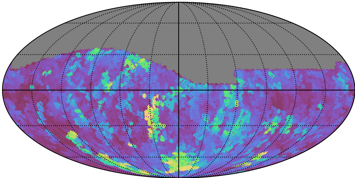
roll_pause_mjdp270_v3.4_10yrs Yr 1 all bands: Max seeingEff
