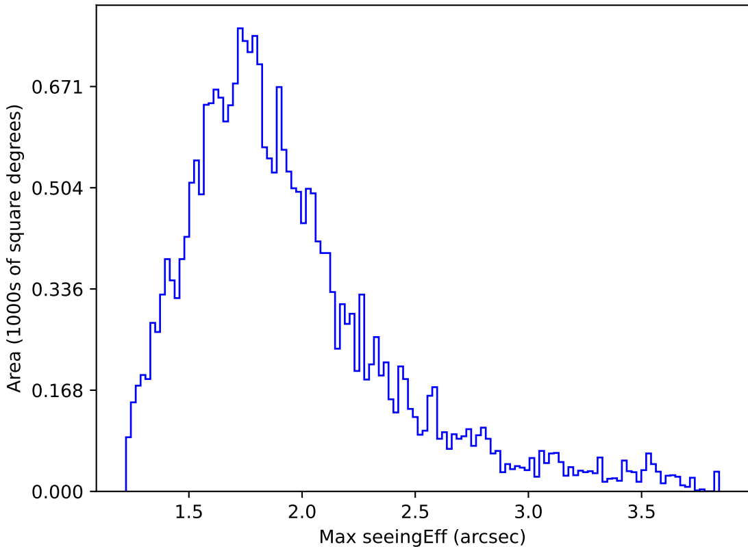
roll_pause_mjdp270_v3.4_10yrs Yr 1 all bands: Max seeingEff
