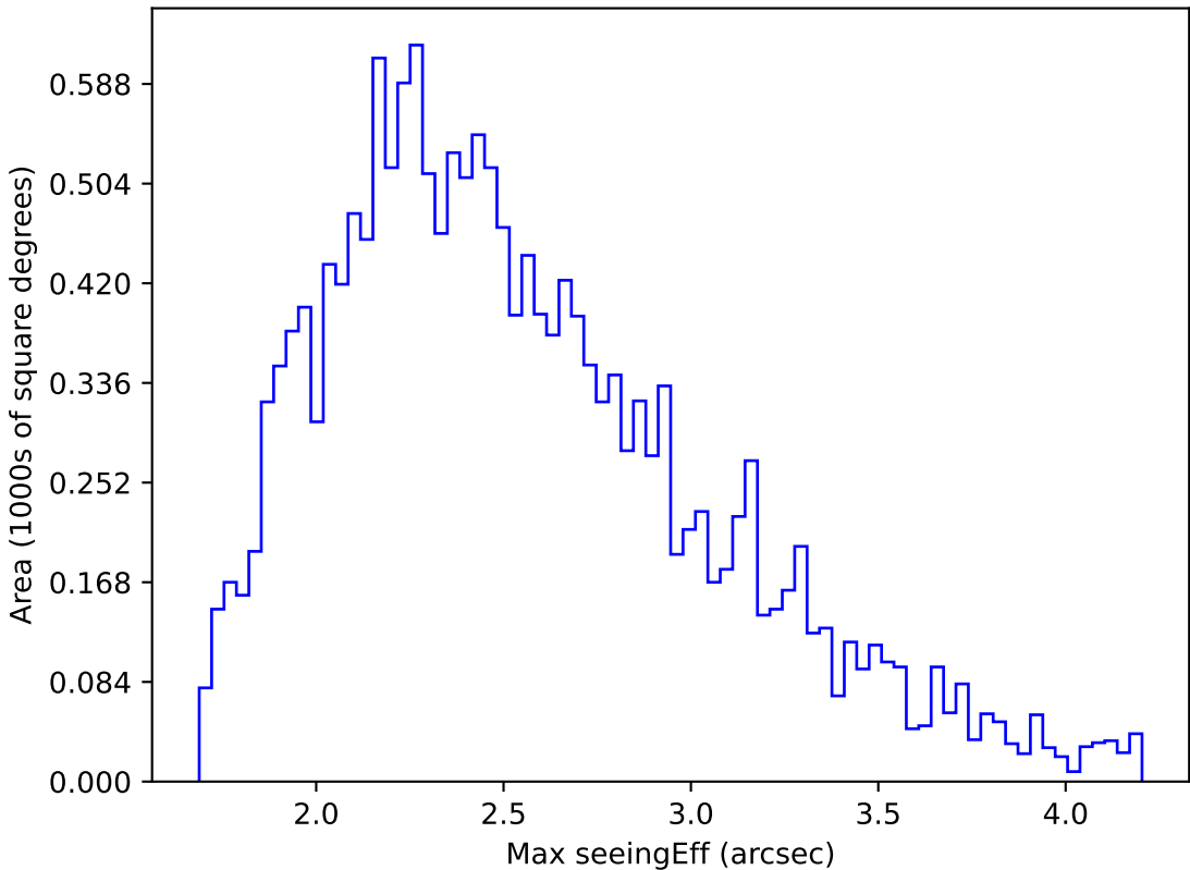
roll_pause_mjdp270_v3.4_10yrs WFD g band: Max seeingEff
