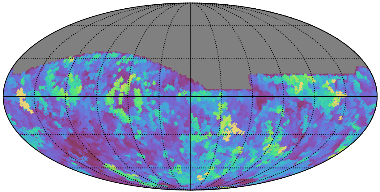
roll_pause_mjdp270_v3.4_10yrs All sky z band: Max seeingEff
