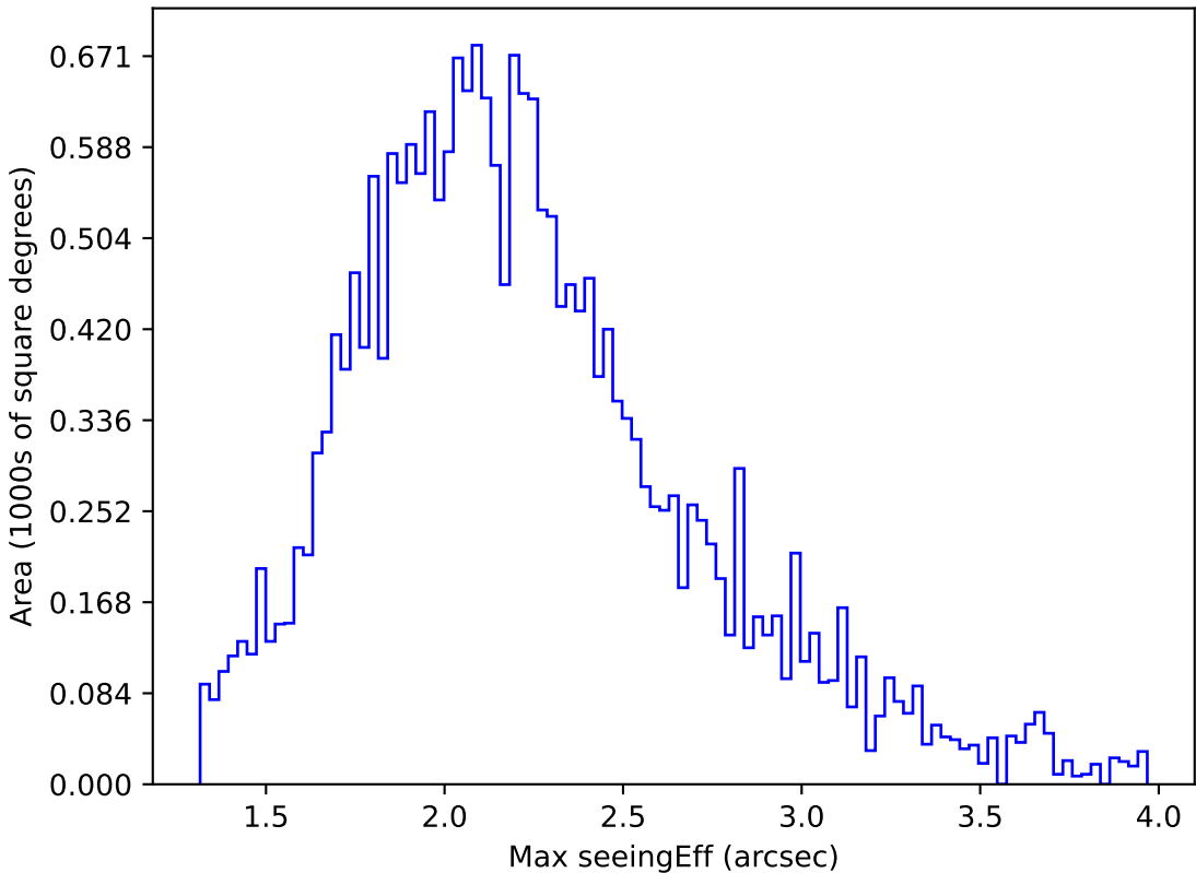
roll_pause_mjdp270_v3.4_10yrs All sky y band: Max seeingEff
