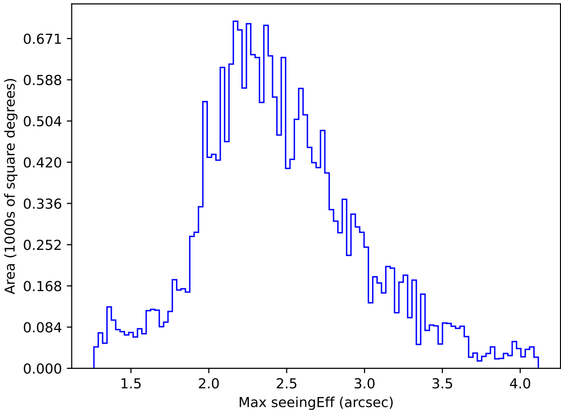
roll_pause_mjdp270_v3.4_10yrs All sky u band: Max seeingEff
