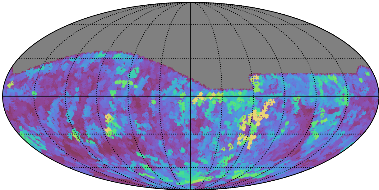
roll_pause_mjdp270_v3.4_10yrs All sky r band: Max seeingEff
