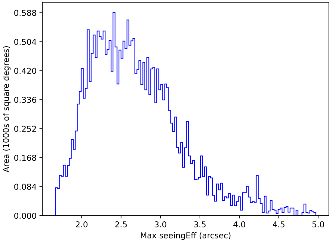
roll_pause_mjdp270_v3.4_10yrs All sky r band: Max seeingEff
