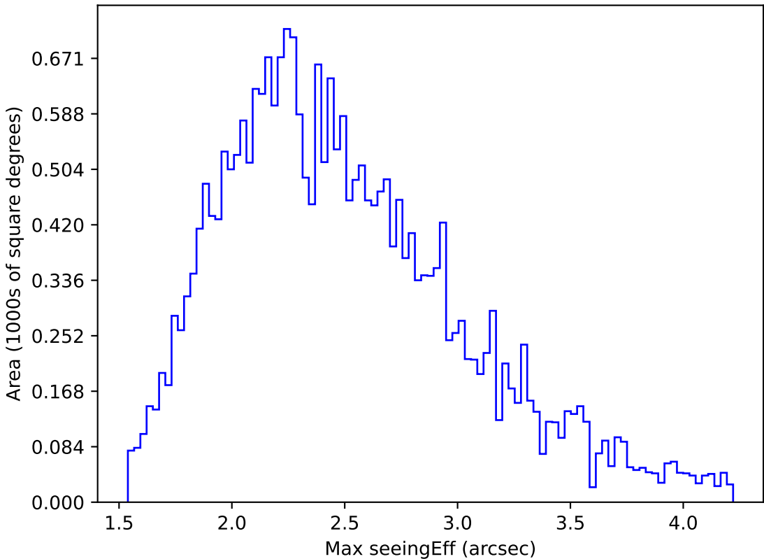
roll_pause_mjdp270_v3.4_10yrs All sky g band: Max seeingEff
