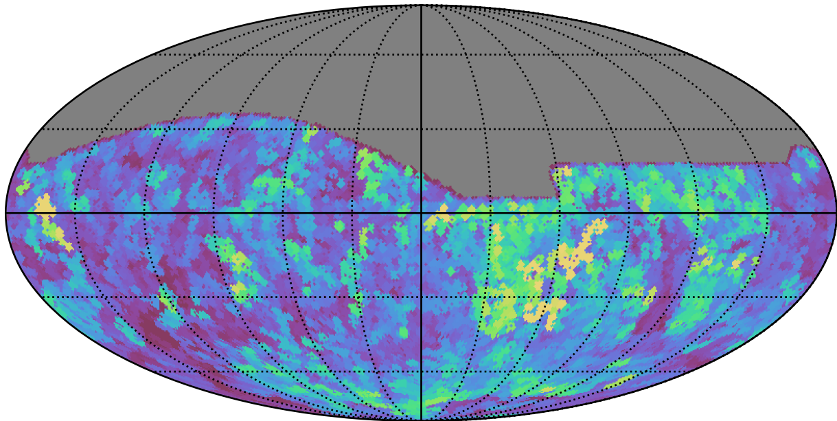
roll_pause_mjdp270_v3.4_10yrs All sky all bands: Max seeingEff
