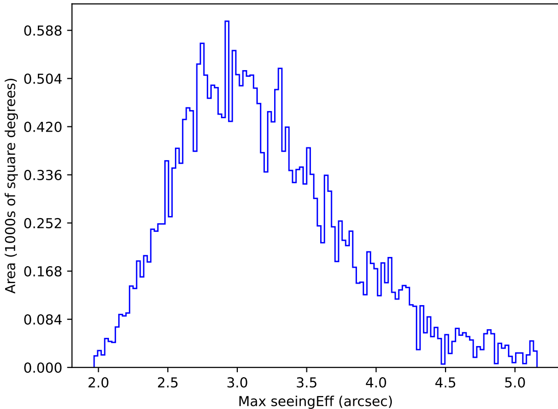
roll_pause_mjdp270_v3.4_10yrs All sky all bands: Max seeingEff
