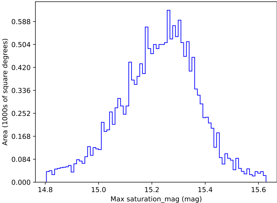
roll_pause_mjdp270_v3.4_10yrs WFD z band: Max saturation_mag
