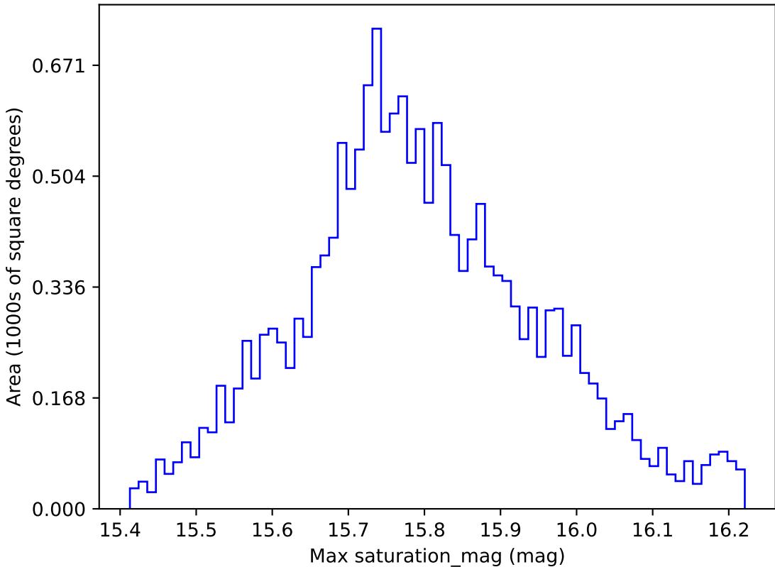
roll_pause_mjdp270_v3.4_10yrs WFD r band: Max saturation_mag
