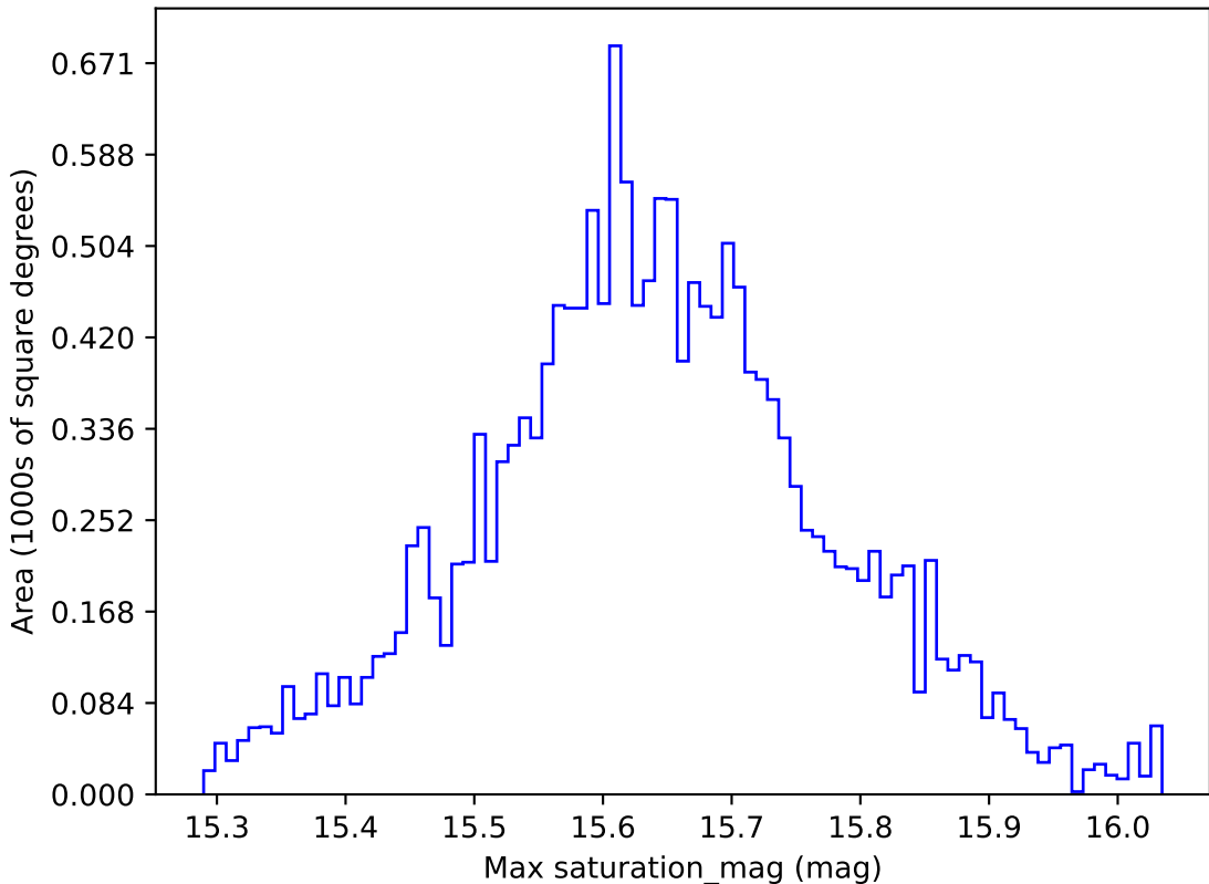
roll_pause_mjdp270_v3.4_10yrs WFD i band: Max saturation_mag
