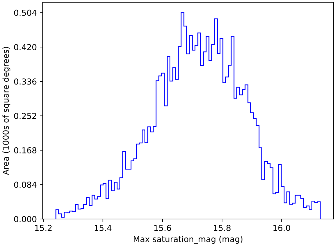
roll_pause_mjdp270_v3.4_10yrs WFD g band: Max saturation_mag
