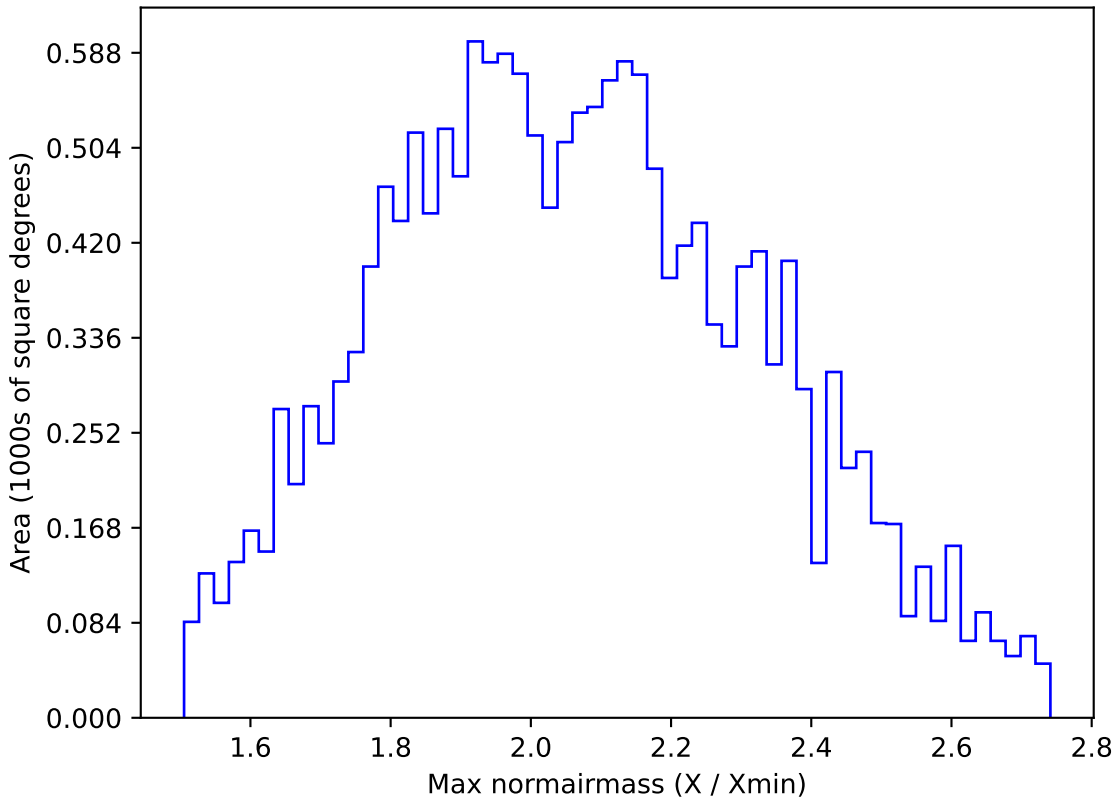
roll_pause_mjdp270_v3.4_10yrs WFD y band: Max normairmass
