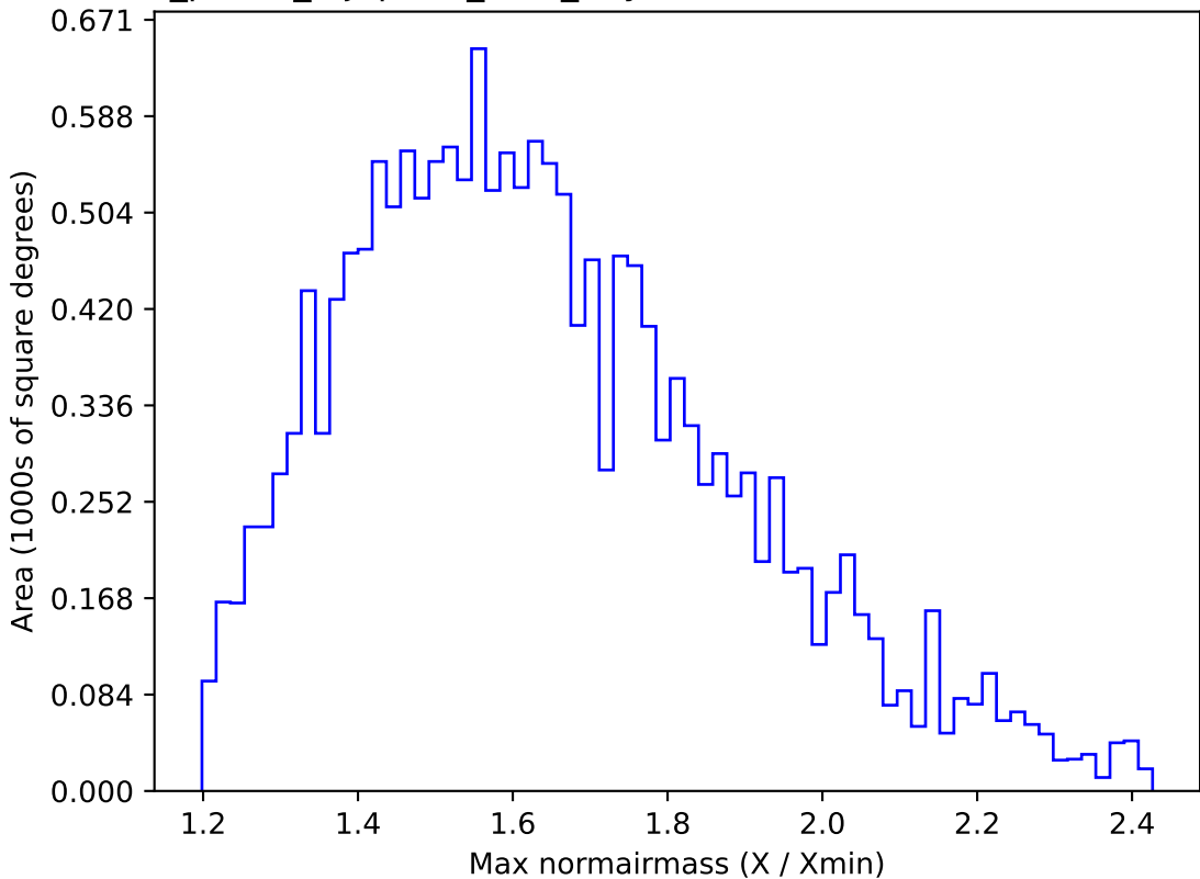
roll_pause_mjdp270_v3.4_10yrs WFD u band: Max normairmass
